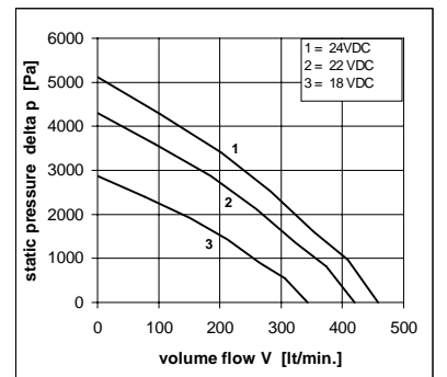
U51DX-024KK-5 24VDC
